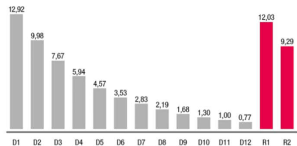
MAN TipMatic 12.28 OD: individual gear ratios
